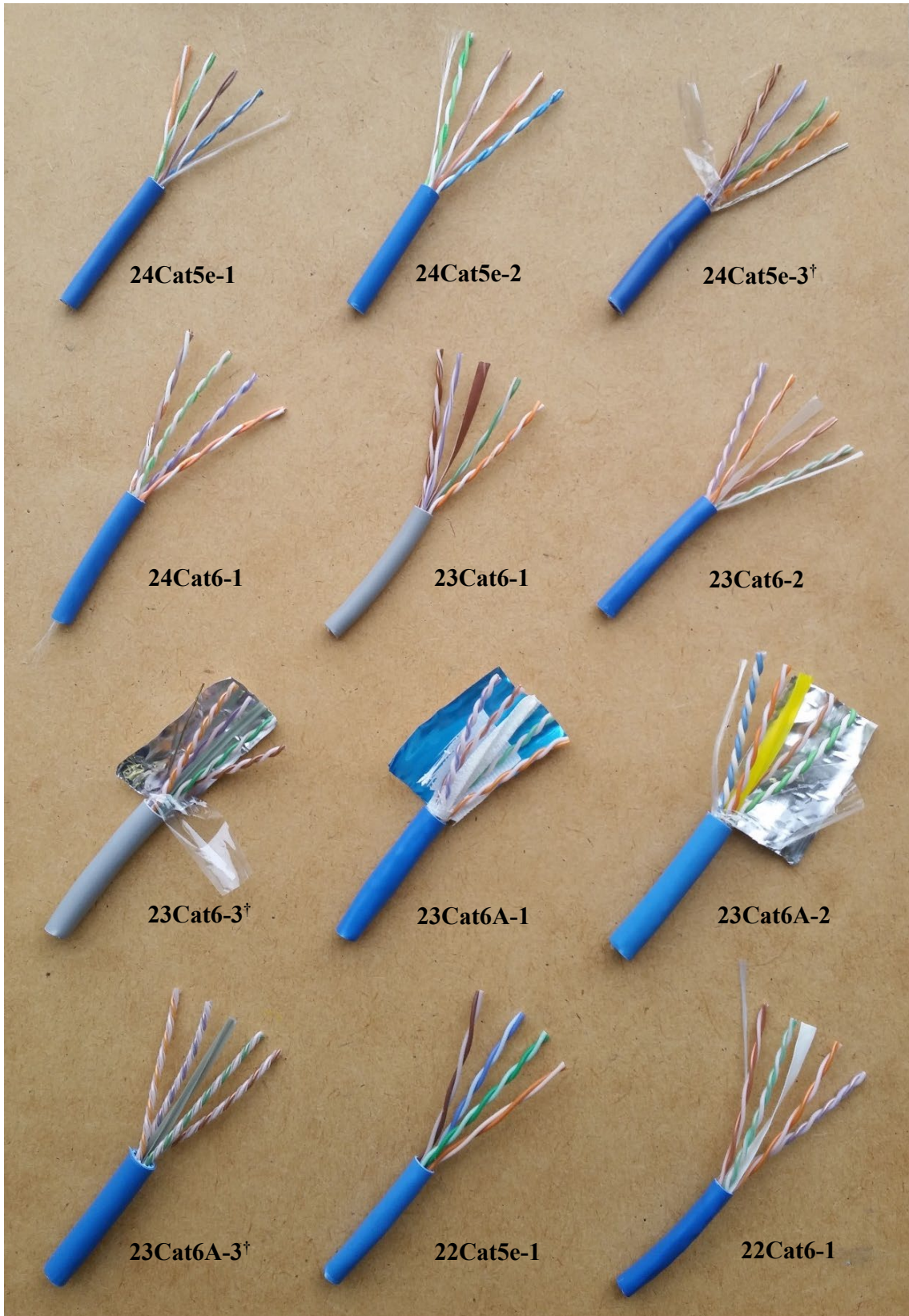
Figure 7.1. The set of cables acquired for testing, each splayed at one end to display internal structure, and shown side-by-side for uniform scale. Labels for the three products removed from testing are marked with a dagger (†) symbol.
