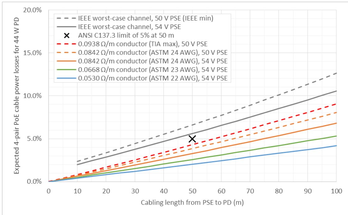
Figure 4. Range of expected 4-pair PoE cable power losses for 44 W PD. The IEEE worst-case channel includes 10 m of patch cord and four connectors (2.6 Ω at 20°C in conditioned space), plus up to 90 m of solid-conductor cable (0.11 Ω/m at 65°C in plenum). Conductor temperature is 20°C for the other five curves.
