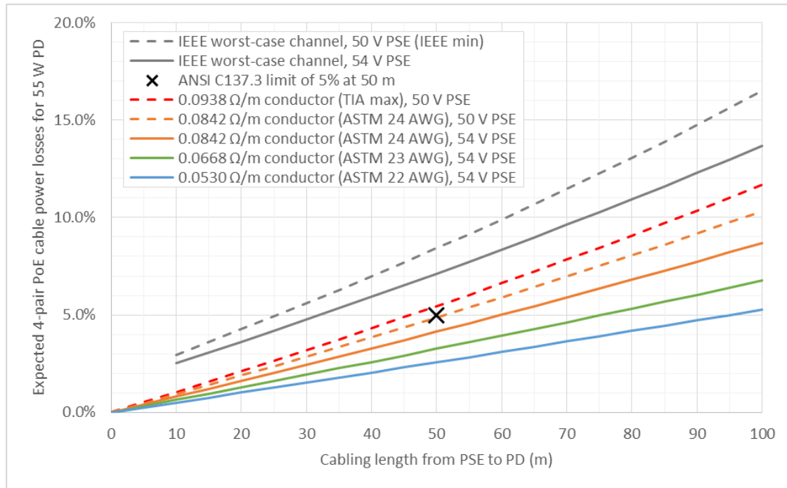
Figure 2. Range of expected 4-pair PoE cable power losses for 55 W PD. The IEEE worst-case channel includes 10 m of patch cord and four connectors (2.6 \Omega at 20 °C in conditioned space), plus up to 90 m of solid-conductor cable (0.11 \Omega /m at 65 °C in plenum). Conductor temperature is 20 °C for the other five curves.
