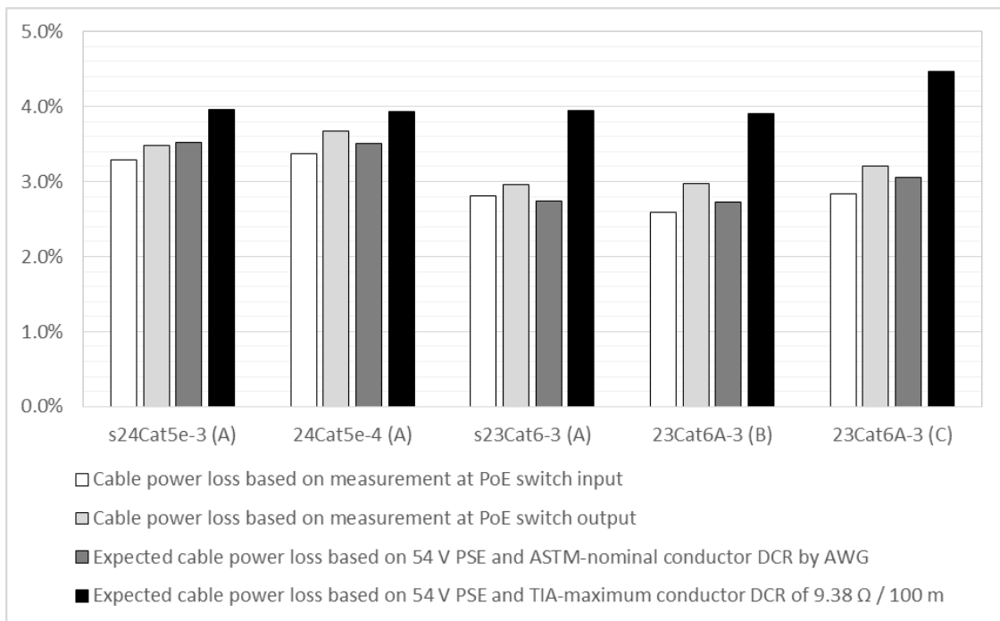
Figure 5. 50 m cable power losses with 44 W PD, based on standard or measured values as shown. X-axis labels indicate test configuration (A, B, or C) in parentheses. Configuration C includes 45 m length cables with two 2.1 m patch cords.
